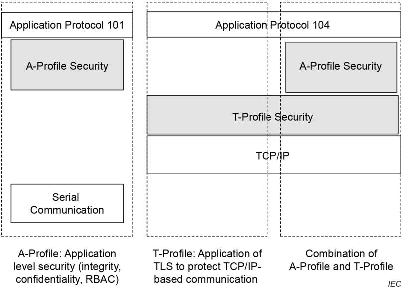
Figure 1 – IEC 60870-5-7 Profiles
