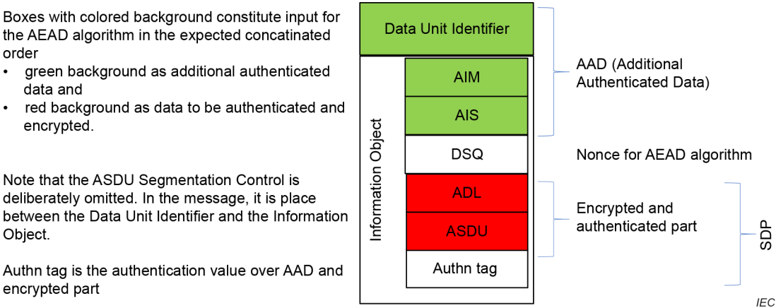
Figure 19 – Example of an AEAD calculation of a Secure Data message
