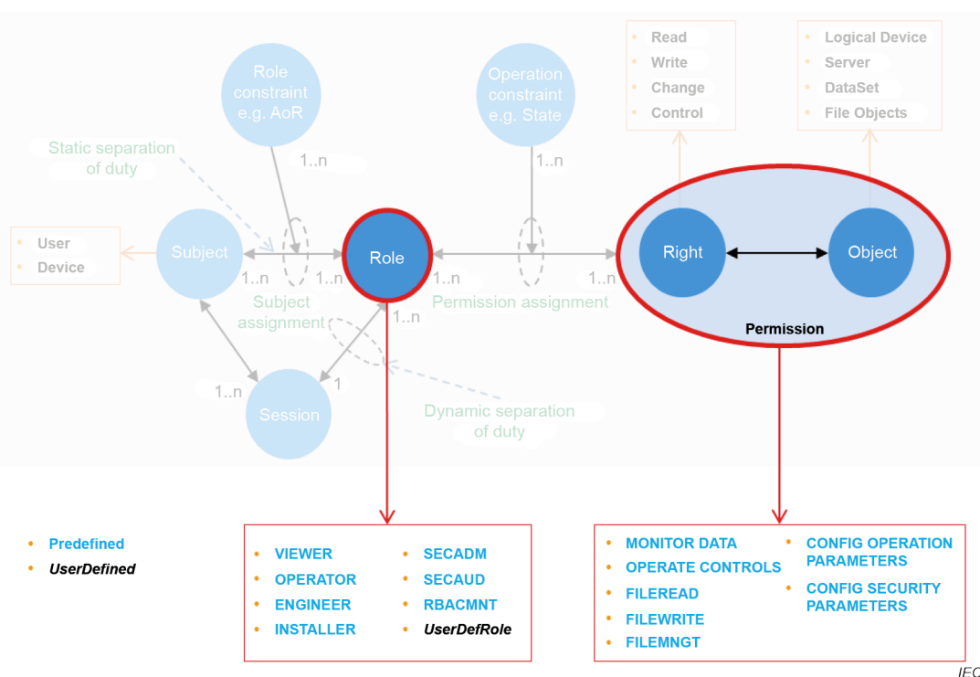
Figure 21 – RBAC mapped to IEC 60870-5-101/-104
