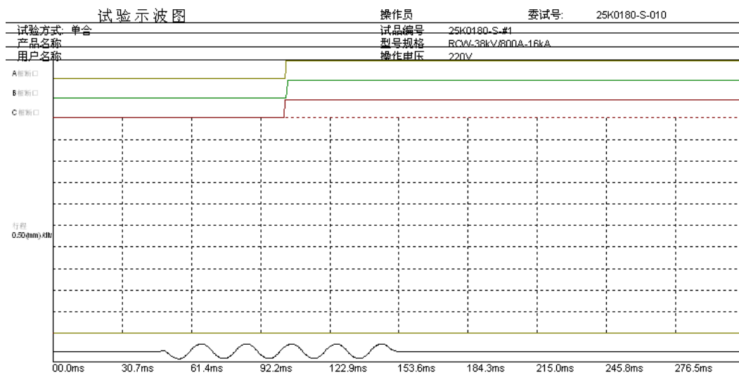
O operation at 220 Vac after 8000 operations mechanical endurance test
