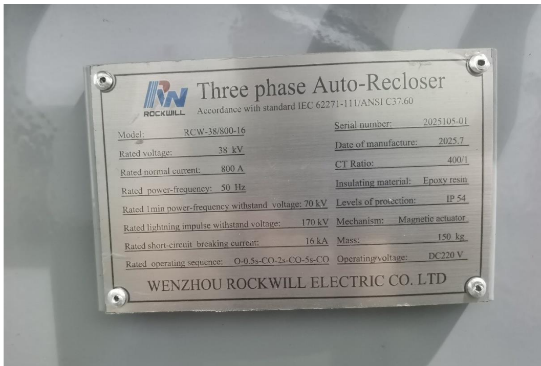
Nameplate
